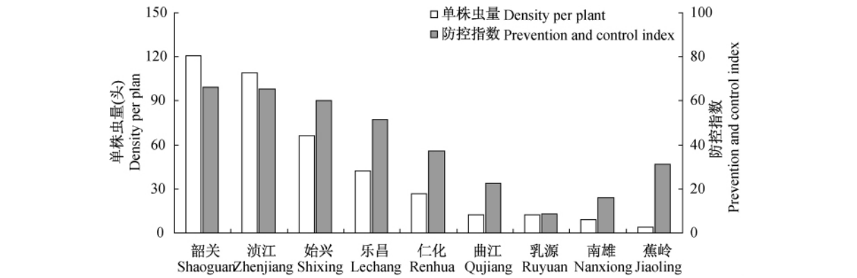
图 2 广东省广聚萤叶甲的单株虫量与防控指数 Fig. 2 The density of O. communa and its prevention and control index in Guangdong Province
