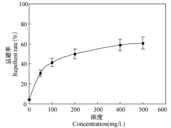
图 2 DPA 对烟粉虱成虫的忌避作用曲线 Fig. 2 Repellence dose-response curve for DPA on B. tabaci adult
