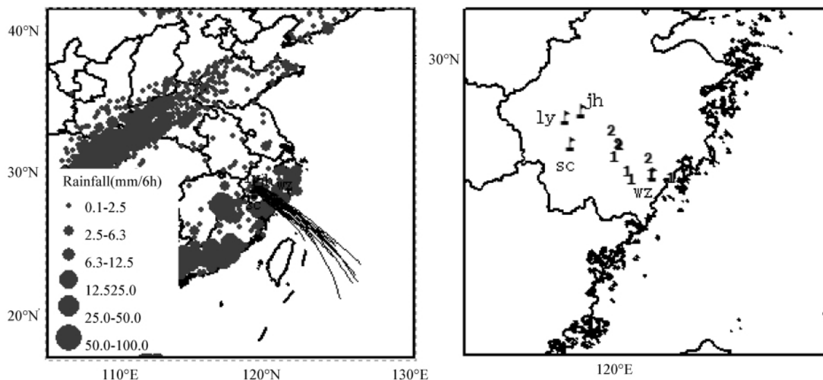
图 3 遂昌(sc)、温州(wz)、龙游(ly) 9 月 9 日回推轨迹(左)和有效终点分布(右)及 9 日 14:00—20:00 降雨分布 Fig. 3 The rainfall distribution during 14:00 to 20:00 and backward trajectories(left) and effective endpoints(right) from Suichang(sc), Wenzhou(wz), and Longyou(ly) on 9 Sep.
