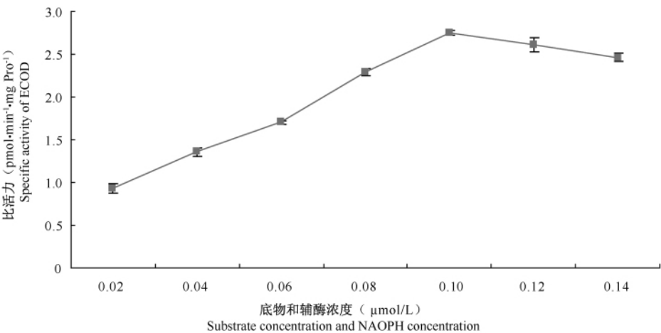
图 1 底物和辅酶浓度对酶比活力的影响 Fig. 1 The effect of substrate concentration and NADPH concentration on the activity of O-deethylation of cytochrome P450
