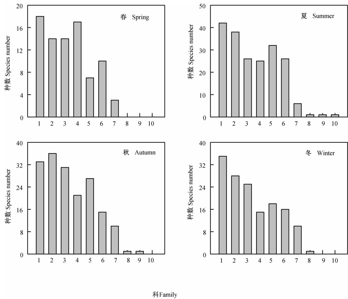
图1 广西桂林雁山地区蝶类季节活动数量变化统计图(2006—2010) Fig.1 The butterflies and their seasonal distribution in Yanshan of Guilin, Guangxi(2006—2010)
