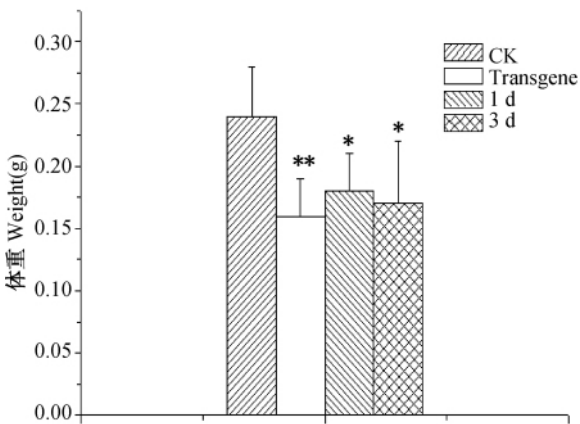
图2 取食不同食物对棉铃虫体重的影响 Fig.2 The comparison of body weight increases of the cotton bollworm larvae fed on different cotton leaves
