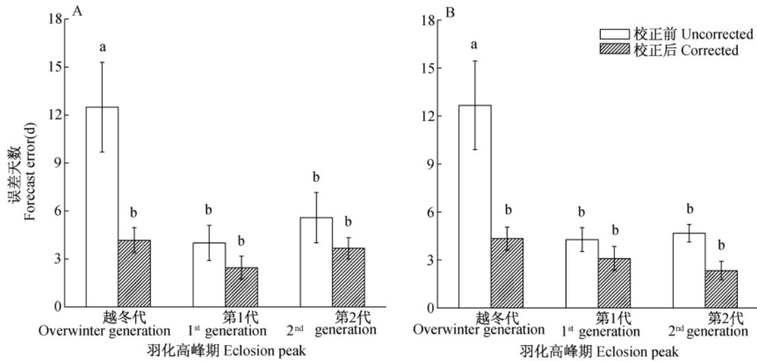
图 3 10 ~ 30℃ (A) 和 10 ~ 35℃ (B) 校正前后有效积温范围预测误差天数比较 Fig.3 Comparison of uncorrected and corrected forecast error days in 10—30℃ (A) and 10—35℃ (B) effective accumulated temperature ranges
