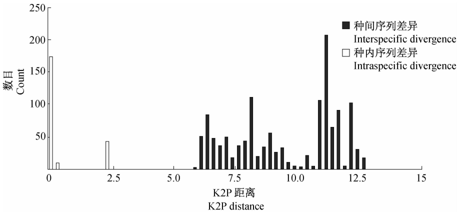
图 5 基于线粒体 COI 658 bp 序列和 K2P 距离的序列差异频次图 (除绣线菊蚜和苹果蚜) Fig.5 Histogram of genetic divergence using mitochondrial COI 658 bp sequences, divergences were calculated using Kimura's two parameter (K2P) model (except A. spiraeicola and A. pomi )
