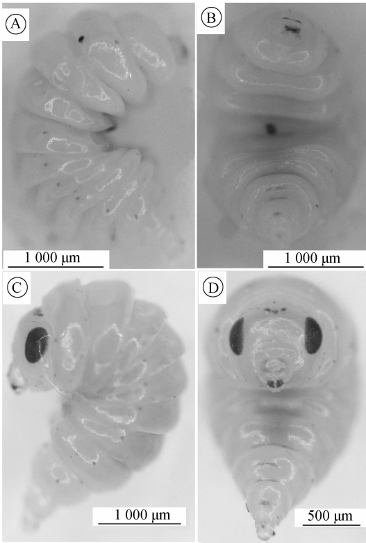
图 1 玫瑰梨癭蜂幼虫形态特征 Fig. 1 Morphology of the larvae of Diplolepis rosae A, B: 2 或 3 龄幼虫形态图 the second or third instar larvae; C, D: 末龄幼虫 the last instar larvae.
