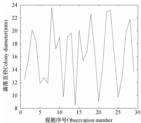
图 2 温度集中时不同温湿度下汤普森被毛孢菌落直径拟合曲线 Fig.2 Fitted curve of Hirsutella thompsonii colony diameter in different humidity when temperature concentrate
