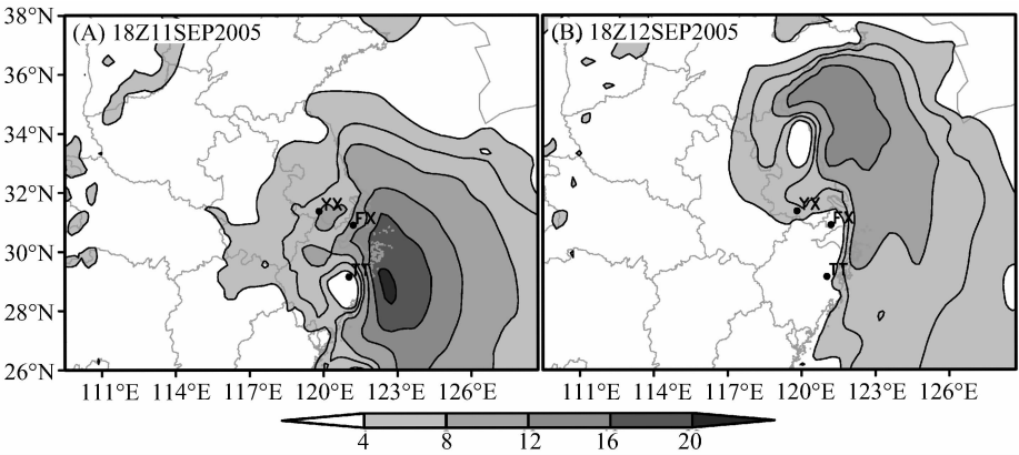
图 4 模拟褐飞虱起飞时刻(18:00)近地面 10 m 的水平风速 (Hu et al. , 2013) Fig.4 The simulated horizontal wind speed at 10 m above ground at 18:00 (shaded, m/s) TT:天台 Tiantai;FX:奉贤 Fengxian;YX:宜兴 Yixing.
