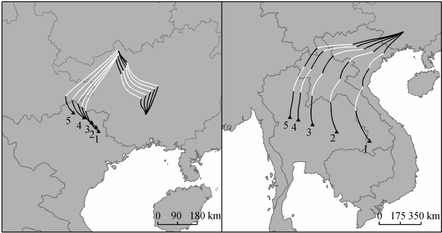
图 2 5 月 6 日 (左) 与 5 月 21 日 (右) 南宁稻纵卷叶螟迁入种群的回推虫源地轨迹 (王凤英等, 2009) Fig. 2 The backward trajectories of the immigratory population of rice leaf roller in Nanning on May 6 (left) and May 21 (right) (from Wang et al. , 2009)
