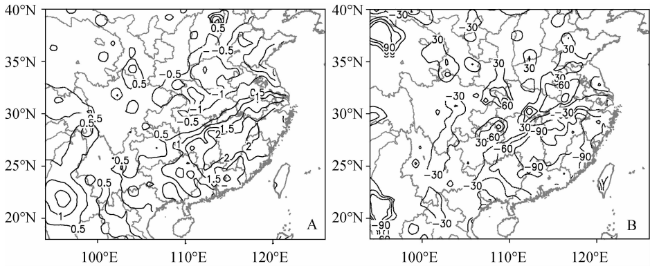
图4 2003年7月中国南方温度距平(A,单位:℃)及降水距平百分率(B,单位:%)分布(气候平均:1961—1990年) Fig.4 Anomalies of temperature (A, unit: ℃) and percentage anomalies of precipitation (B, unit: %) in July, 2003 in southern China (from the mean between 1961 and 1990)
