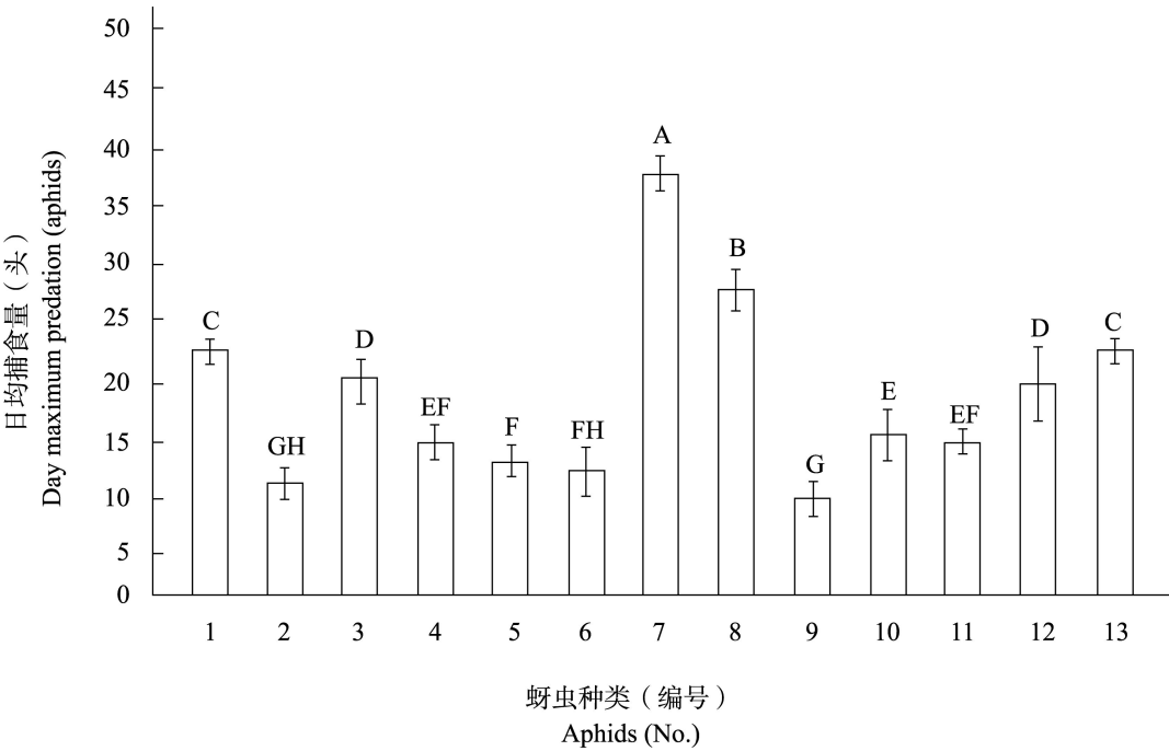
图 1 双七瓢虫 4 龄幼虫对不同蚜虫的日均捕食量 Fig. 1 The day maximum predation of 4th instar larvae in Coccinula quatuordecimpustulata on aphids 柱上标有不同字母表示在 0.05 水平差异显著。下图同。 Histograms with different letters indicate significantly different at the 0.05 level by LSD test. The same below.
