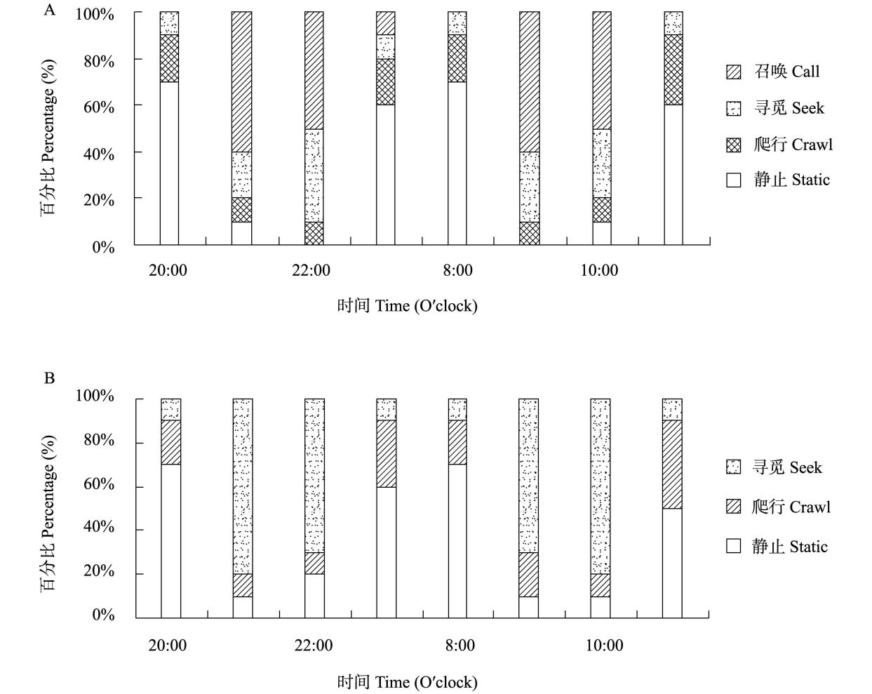
图 2 成虫活跃期活动节律 Fig. 2 The rhythm of alates activity in rush hours
