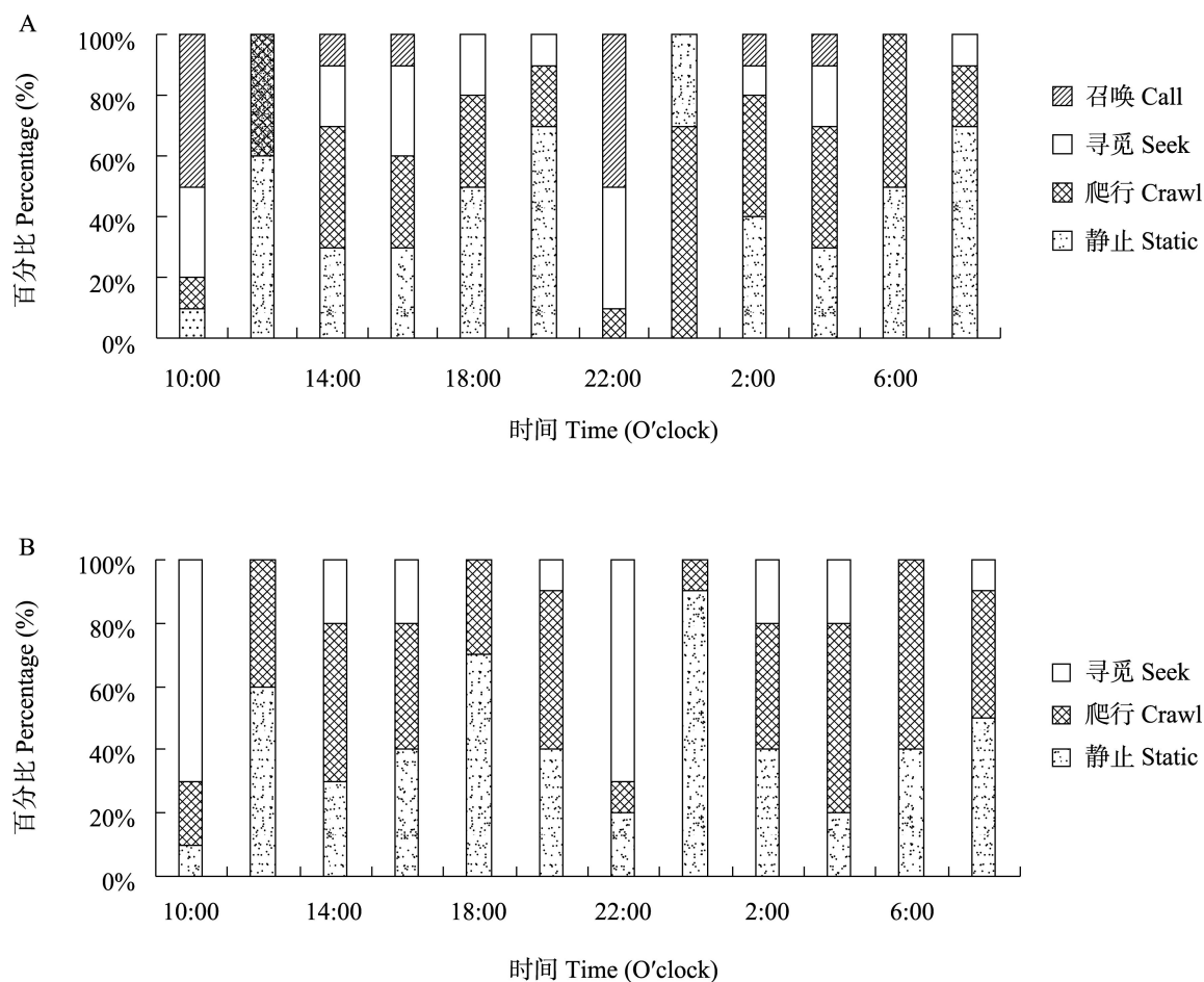
图 1 成虫行为时辰节律 Fig. 1 The 24-hour circadian rhythm of alates behavior
