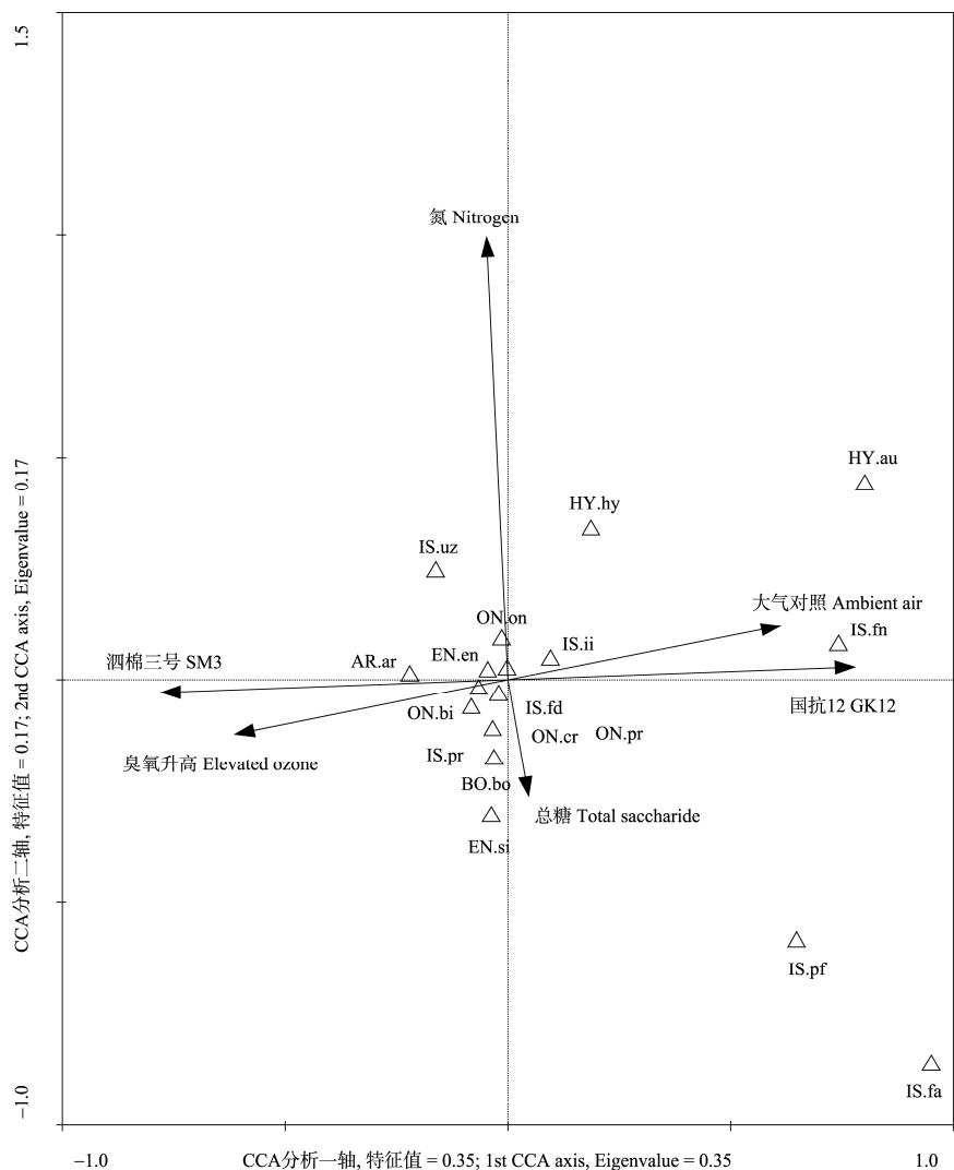
图 1 典范对应分析不同臭氧浓度 (大气对照和臭氧升高) 和棉花品种 (转基因棉国抗 12 和亲本对照泗棉三号) 凋落物中跳虫平均数与环境因子之间的关系 Fig. 1 Ordination biplot of canonical correspondence analysis (CCA), with the mean abundances of soil Collembola in the litters of different ozone concentration (ambient air and elevated ozone) and cotton variety (transgenic Bt cotton GK12 and its near-isolines SM 3)
