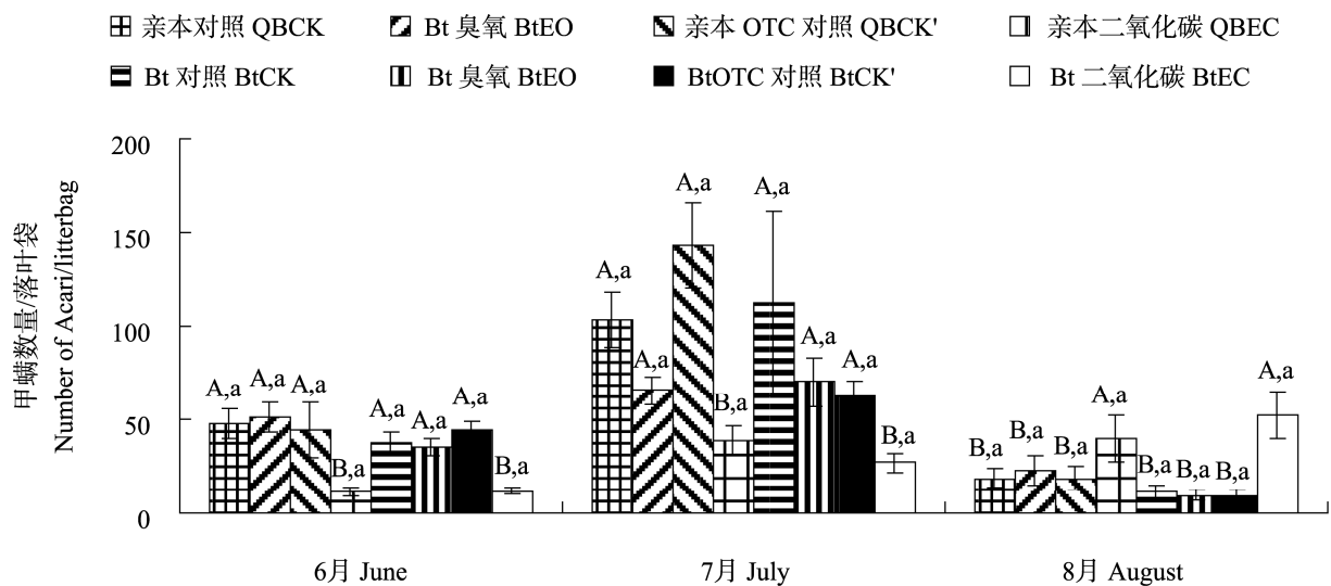
图 2 棉花凋落物内螨类在不同棉花生长期 (8 个样地中的平均值) Fig. 2 Number of soil Acari (mean of two cotton varieties, elevated CO 2 , elevated O 3 , atmospheric atmosphere and open-top chamber control levels) per field ( n = 8 ) of the litterbag study
