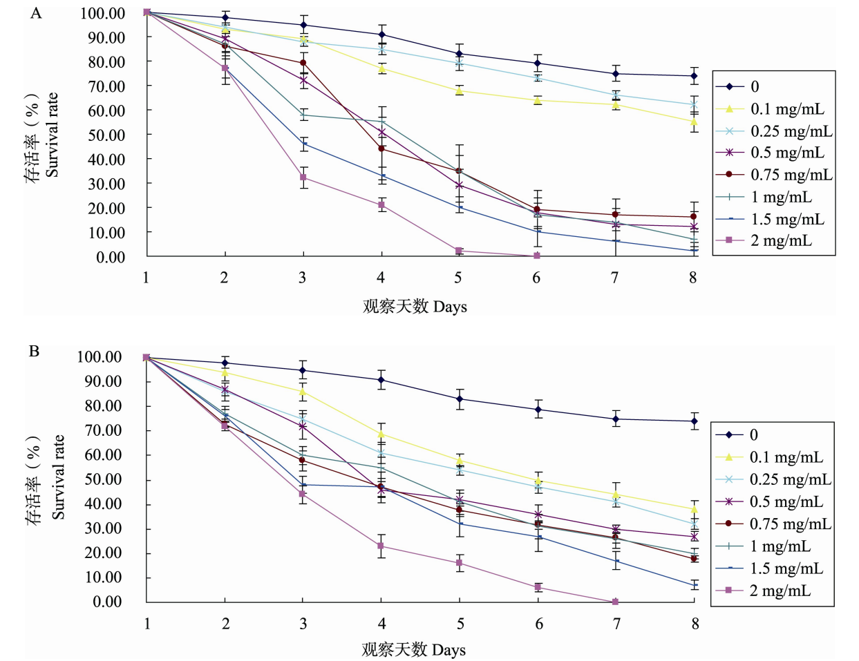
图 11 两种植物凝集素对麦长管蚜存活率的影响 Fig. 11 The effects of two lectins on the survival rate of Sitobion avenae
