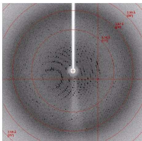
图 8 CYP337B3 ( \Delta 23 ) 晶体衍射图 Fig. 8 The typical X-ray diffraction pattern from a CYP337B3 ( \Delta 23 ) crystal
