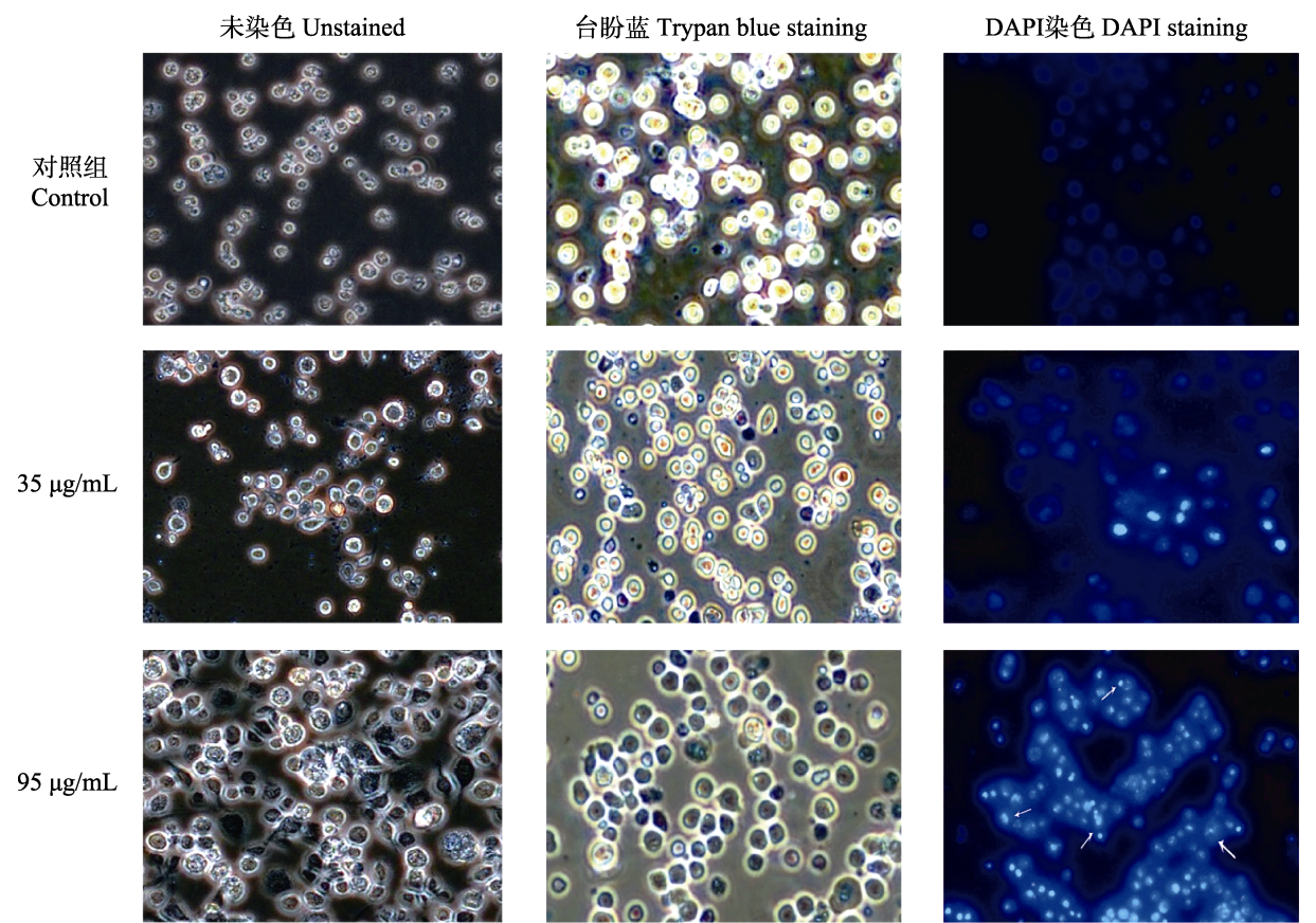
图 1 倒置显微镜下正常 S2 细胞和对硫磷处理细胞的形态变化及细胞凋亡 Fig. 1 Morphological changes and apoptosis in S2 cells induced by parathion, observed by inverted phase contrast microscope
