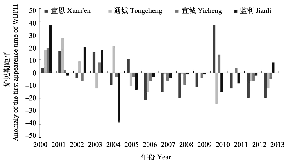
图 2 2000—2013 年湖北白背飞虱前期迁入种群灯诱始见期距平逐年变化图 Fig. 2 Annual anomalies form the year 2000 to 2013 for the first appearance time of WBPH light-trap catches in Hubei Province
