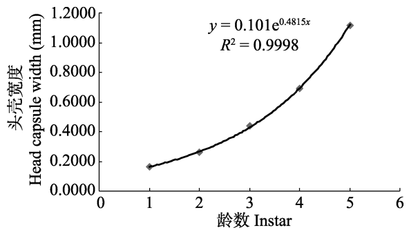
图 2 法氏柴胡宽蛾幼虫虫龄与头壳宽度的回归关系 Fig. 2 Regression relationship between larval instar and head capsule width in Depressaria falkovitshi larvae
