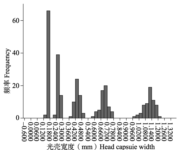
图 1 法氏柴胡宽蛾幼虫头壳宽度频次分布图 Fig. 1 Frequency distribution of head capsule width in Depressaria falkovitshi larvae
