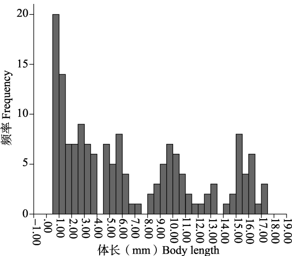
图 3 法氏柴胡宽蛾幼虫体长频次分布图 Fig. 3 Frequency distribution of body length in Depressaria falkovitshi larvae
