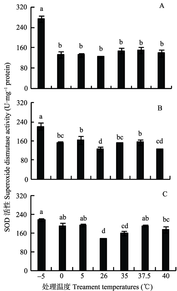
图 1 温度胁迫对 SOD 活性的影响 Fig. 1 Superoxide dismutase activity of Darna trima exposed to temperature stresses
