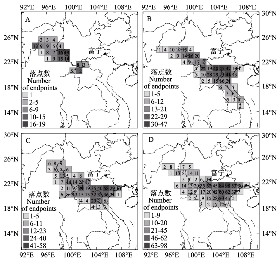
图 2 2008—2012 年 4—5 月富宁白背飞虱虫源地分布 Fig. 2 The distribution of source area of immigrating WBPH in Funing in April and May during 2008 to 2012 A. 4 月; B. 5 月上旬; C. 5 月中旬; D. 5 月下旬。 A. April; B. The first ten days of May; C. The second ten days of May; D. The last ten days of May.
