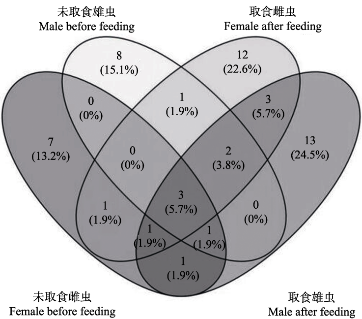
图 1 取食前后丽蝇蛹集金小蜂雌、雄虫体内分可培养真菌数量 Fig. 1 The number of feeding on culturable fungi communities between female and male adults of Nasonia vitripennis
