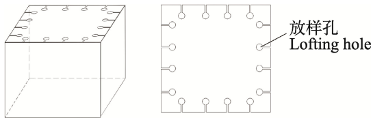
图 3 放样台整体及顶面示意图 Fig. 3 Sketch of whole and the top surface of the lofting platform
