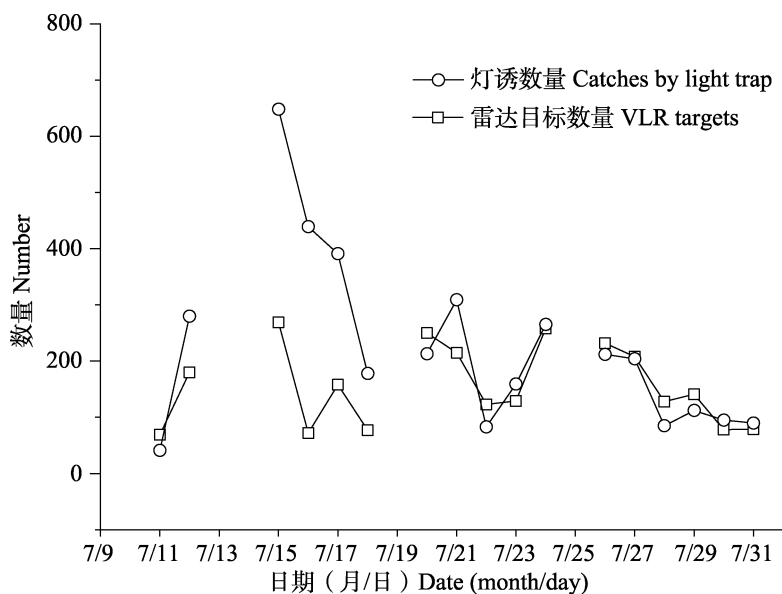
图 2 7 月每日灯诱二点委夜蛾数量和雷达观测的二点委夜蛾 (13.2-44.52 mg) 目标 Fig. 2 Daily aerial densities of Athetis lepigone moths in light trap and the mean daily aerial numbers of Athetis lepigone moth-like targets (13.2-44.52 mg) detected by VLR in July
