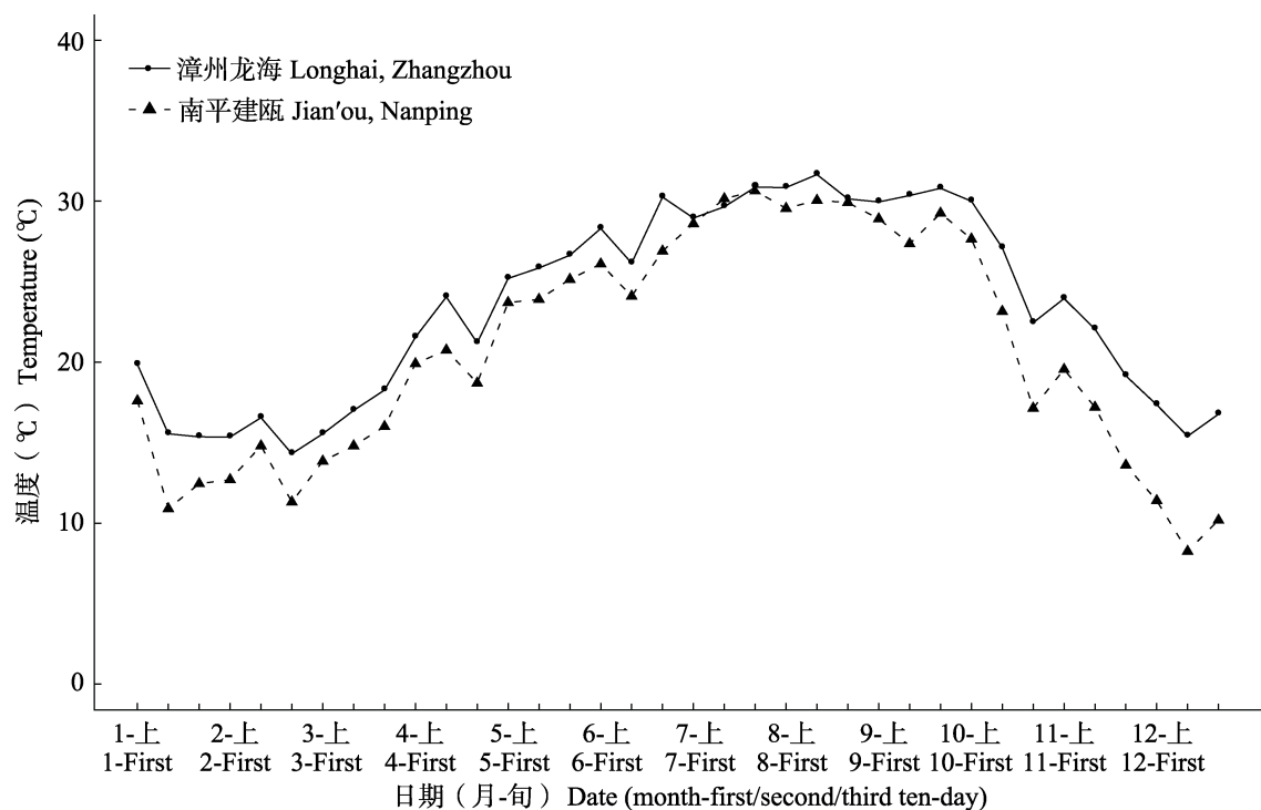
图 2 福建省漳州和南平 2017 年旬平均气温变化曲线 Fig. 2 Change curves of the 10 days' average temperature during 2017 in Fujian 上：上旬。First: First 10 days.
