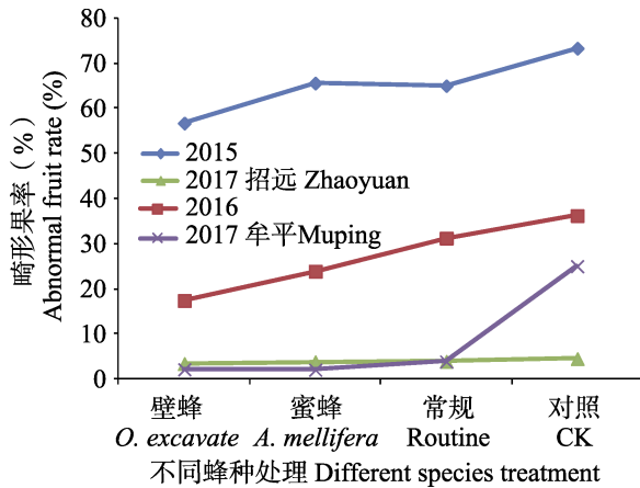
图 4 2015-2017 年不同处理下苹果的畸形果率 Fig. 4 Comparison of abnormal fruit rate of apple by different treatment from 2015 to 2017
