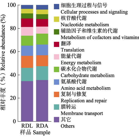
图 4 谷蠹幼虫和成虫体内细菌基因功能注释相对丰度柱形图 Fig. 4 Relative abundance and gene function annotation of the bacteria in larvae and adults of Rhyzopertha dominica
