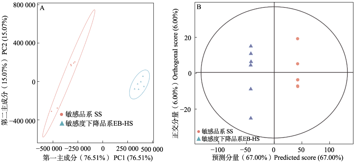
图 5 草地贪夜蛾 SS 和 EB-HS 中代谢物的主成分分析得分图 (A) 及正交偏最小二乘判别分析得分图 (B) Fig. 5 Principal component analysis score plot (A) and orthogonal partial least squares discriminant analysis score plot (B) of metabolites in SS and EB-HS of Spodoptera frugiperda
