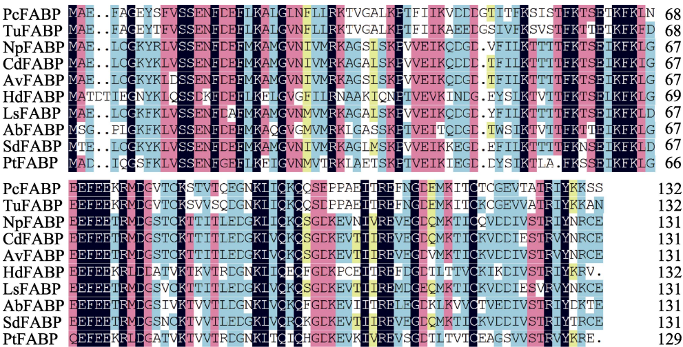
图 2 柑橘全爪螨 PcFABP 氨基酸序列与其他物种氨基酸序列的比对 Fig. 2 Multiple alignments of PcFABP amino acid sequences of Panonychus citri and other species 蓝色代表 100%序列一致性,红色代表≥75%序列一致性,绿色代表≥50%序列一致性,黄色代表≥33%序列一致性。 Blue represents 100% identity, red represents≥75% identity, green represents≥50% identity and yellow represents≥33% identity.
