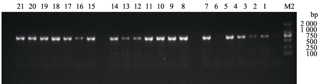
图 3 酒精保存样本中 3 种方法提取的基因组 DNA 的 PCR 电泳结果 Fig. 3 PCR electrophoresis results of genomic DNA extracted by three methods preserved samples in alcohol
