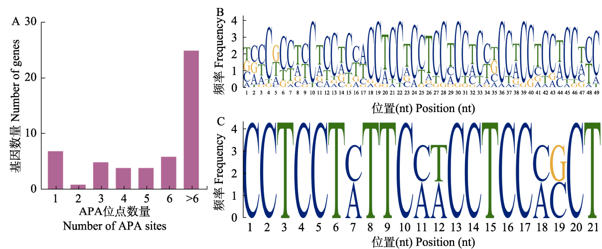
图 1 意大利蜜蜂 MAPK 信号通路相关基因 APA 位点分布特性的统计与分析 Fig. 1 Statistics and analysis of APA sites within genes associated with MAPK signaling pathway in Apis mellifera ligustica
