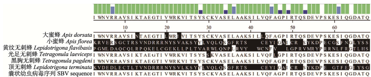
图 3 6 种野生蜂 SBV 片段与西方蜜蜂的氨基酸序列对比 Fig. 3 Comparison of amino acid sequences of SBV fragments of six wild bees
